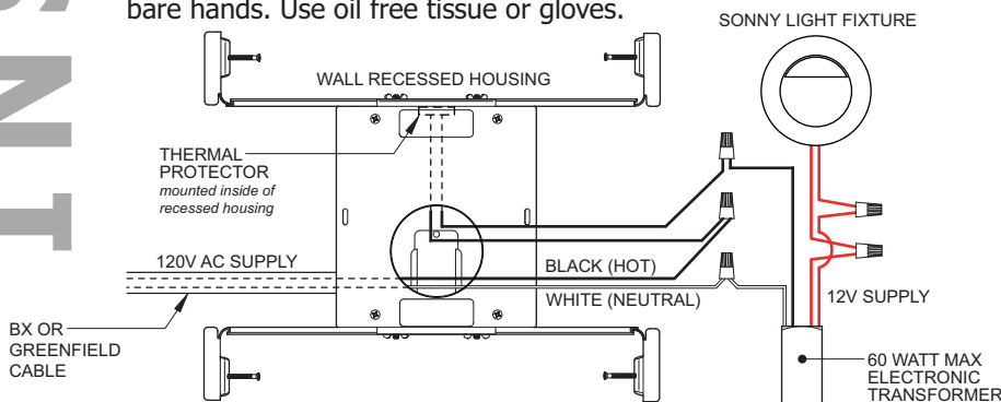
SONNY LIGHT FIXTURE - image shown with faceplate removed for relamping.
