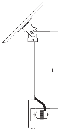
M2P-4RD-SL2-SN Monorail 2-Circuit 4" Round Power Feed Canopy with 2" Slope shown.
